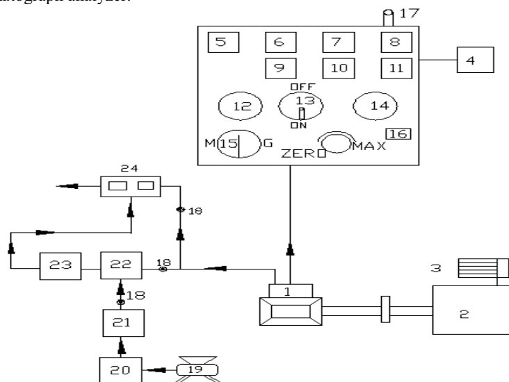
1. Engine, 2. Electrical swinging field dynamometer, 3. Loading arrangement, 4. Fuel tank, 5. Torque indicator/controller sensor, 6. Fuel rate indicator sensor, 7. Hot wire gas flow indicator, 8. Multi channel temperature indicator, 9. Speed indicator, 10. Air flow indicator, 11. Exhaust gas temperature indicator, 12. Mains ON, 13. Engine ON/OFF switch, 14. Mains OFF, 15. Motor/Generator option switch, 16. Heater controller, 17. Speed indicator, 18. Directional valve, 19. Air compressor, 20. Rotometer, 21. Heater, 22. Air chamber, 23. Catalytic chamber, 24. CO/HC analyzer,
