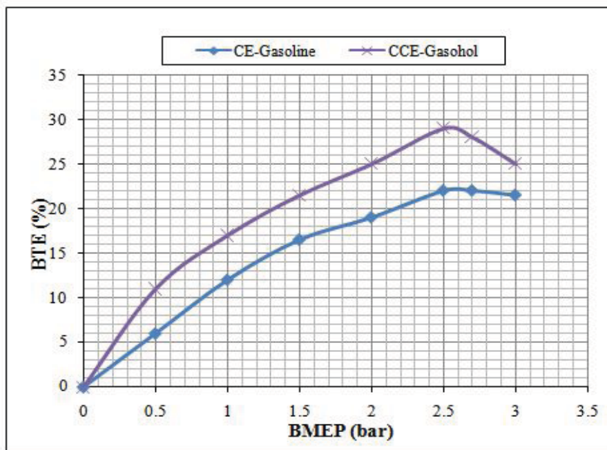
CE- conventional engine; CCCC-Copper coated combustion chamber. BTE- brake thermal efficiency BMEP-Brake mean effective pressure
