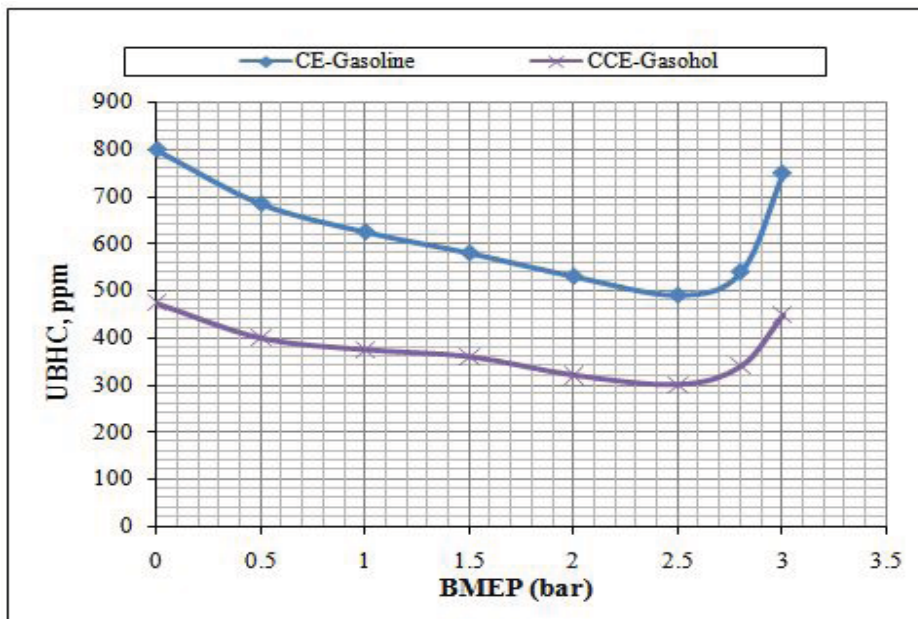
CE- conventional engine: CCCC-Copper coated combustion chamber, UBHC- Un-burnt hydro carbons: BMEP-Brake mean effective pressure
