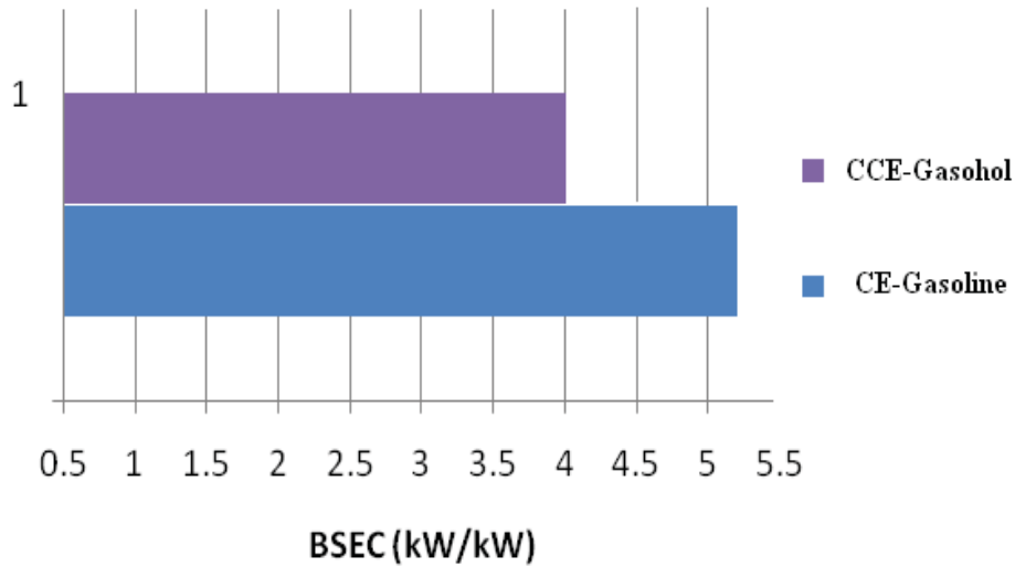
Figure.4 presents bar charts showing the variation of brake specific energy consumption (BSEC) at full load operation with different versions of the combustion chamber with test fuels
