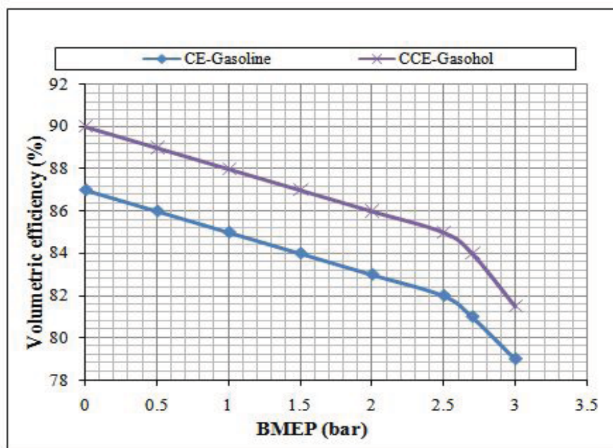
CE- conventional engine; CCCC-Copper coated combustion chamber, BMEP-Brake mean effective pressure Figure.6 Variation of volumetric efficiency with BMEP in different versions of the combustion chamber with test fuels at a compression ratio of 7.5:1 and speed of 3000 rpm
