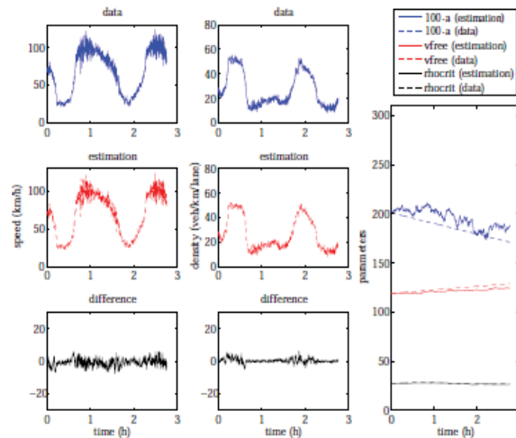
Fig. 3. State and parameter estimation with the joint EKF, all segments are measured.
