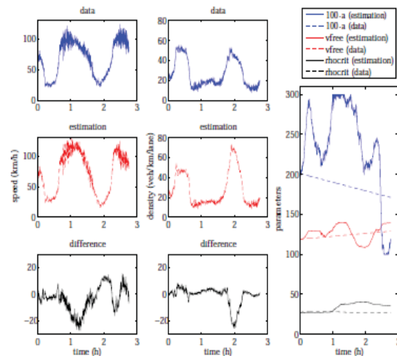
Fig. 4. State and parameter estimation with the dual EKF, all segments are measured.
