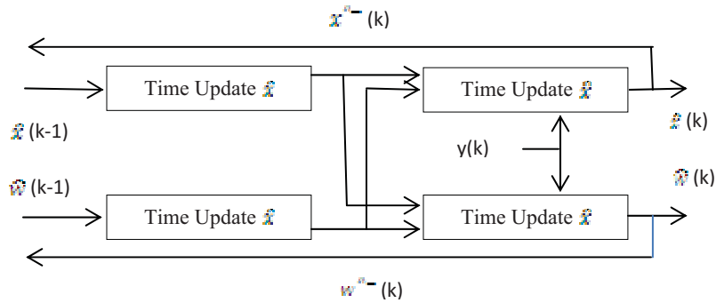
Fig. 1.The dual estimation scheme. The two filters use each other's estimation from the previous sample step.
