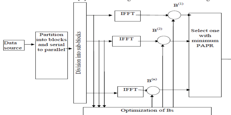
Figure-1: Block diagram of PTS technique
