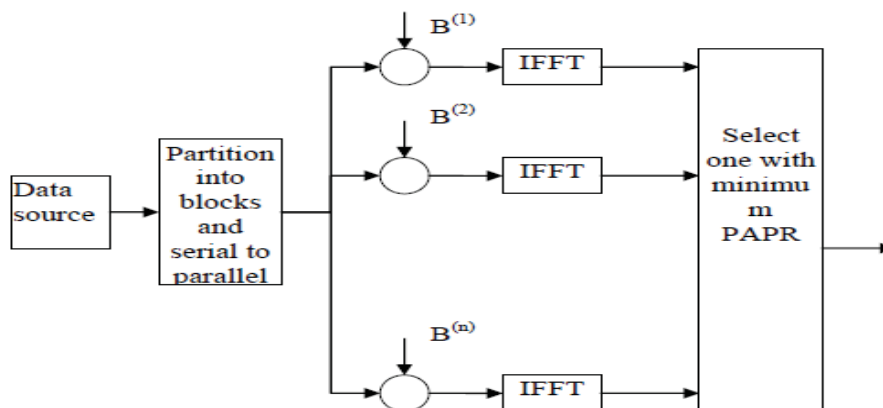
Figure-2: Block diagram of SLM technique.
