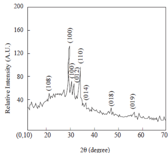
Figure1. X-ray diffraction pattern of Bismuth oxide thin films deposited on glass substrates.
