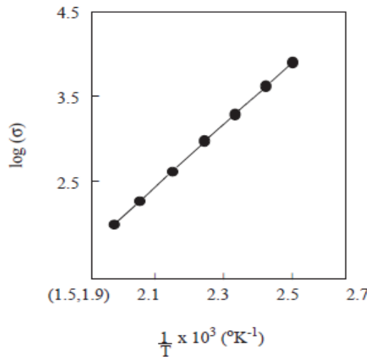
Figure 4. ariation of log(σ) versus 1/T for bismuth oxide thin films.
