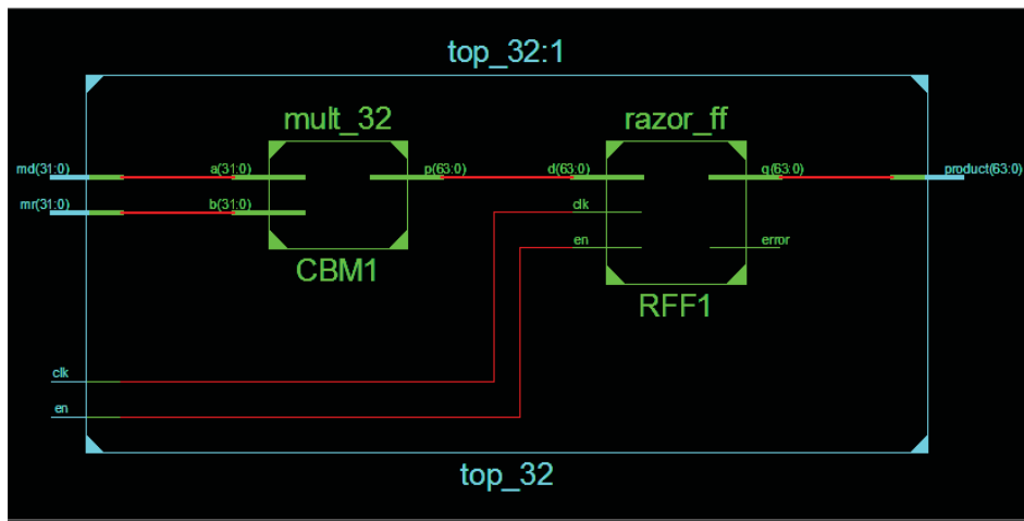
Figure 8.RTL schematic.
