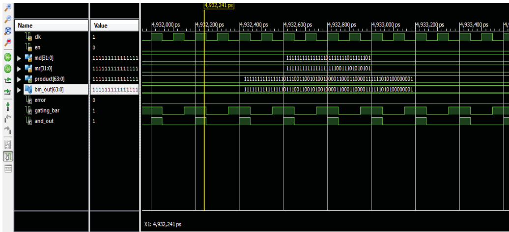
Figure 7.Simulation Results.
