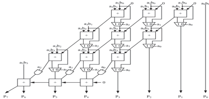
Figure 2. 4 X 4 column_bypassing multiplier
