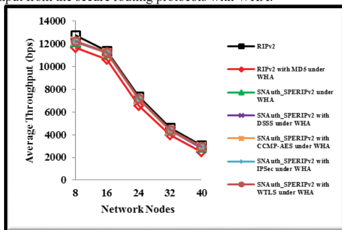
Figure5 (d): Average throughput versus number of network nodes
