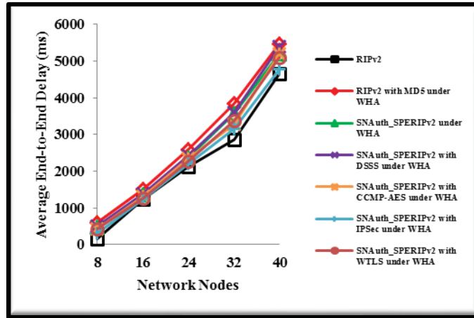
Figure5 (e): Average end-to-end delay versus number of network nodes
