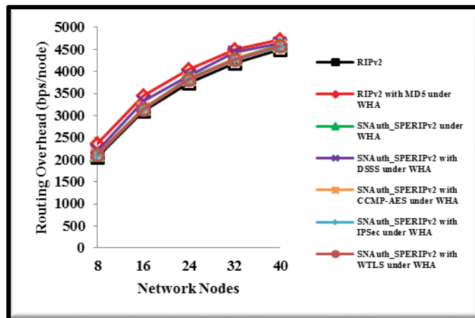
Figure4 (b): Average routing overhead versus number of network nodes
