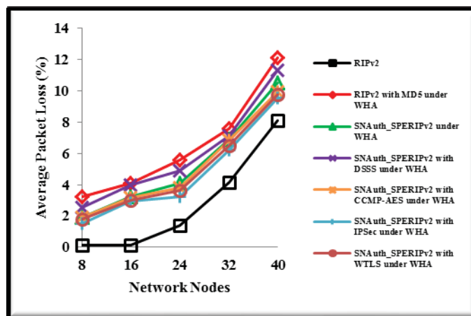
Figure4 (c): Average packet loss versus number of network nodes
