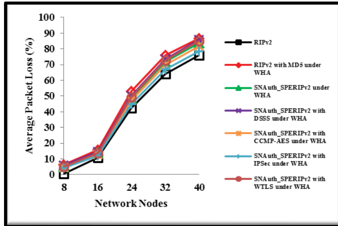
Figure5(c): Average packet loss versus number of network nodes
