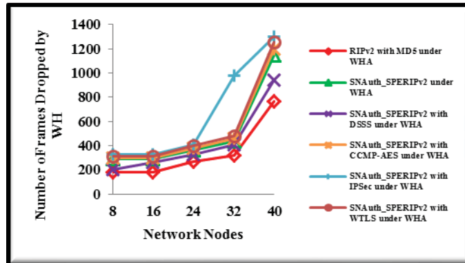
Figure5 (a): Number of frames dropped by WH versus number of network nodes
