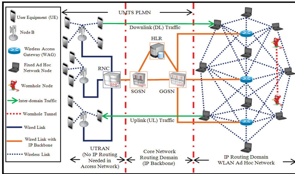
Figure 3. The Integrated UMTS and WLAN Ad Hoc network with WH adversary
