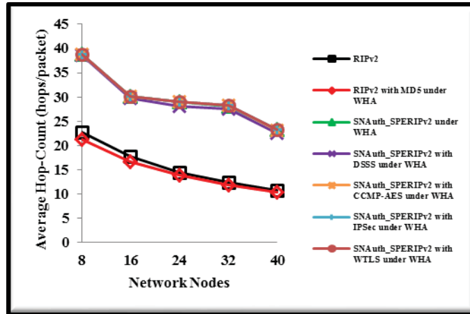
Figure5 (g): Average hop-count versus number of network nodes
