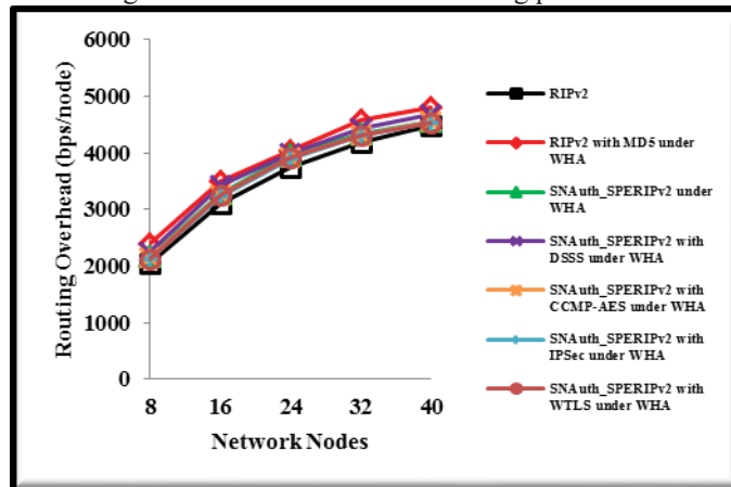
Figure5 (b): Average routing overhead versus number of network nodes
