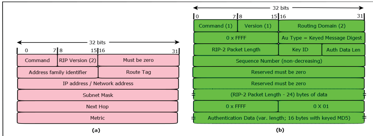
Figure 2. RIPv2 message format (a) with plain text password (b) keyed MD5
