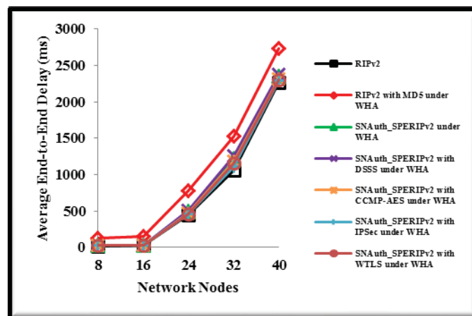
Figure4 (e): Average end-to-end delay versus number of network nodes
