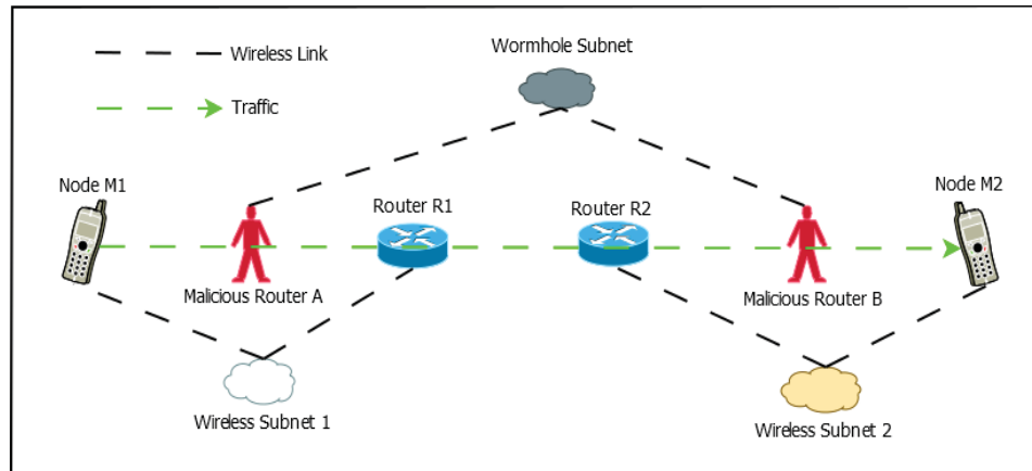
Figure 1. The WH adversary under transparent mode
