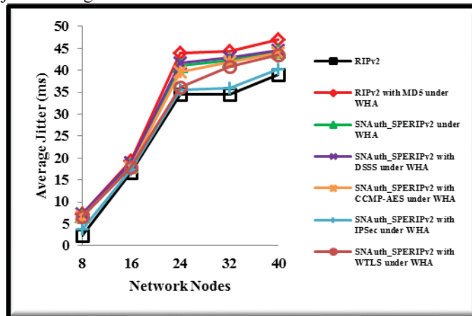
Figure5 (f): Average jitter versus number of network nodes
