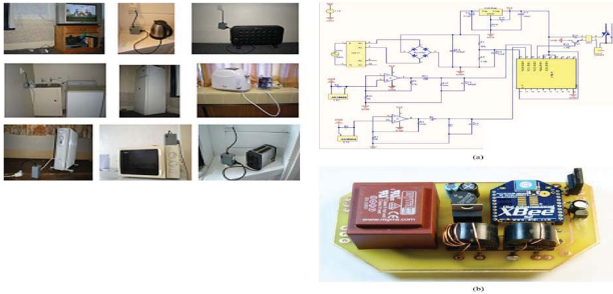
Fig. 2 Developed system with different electrical appliances.
