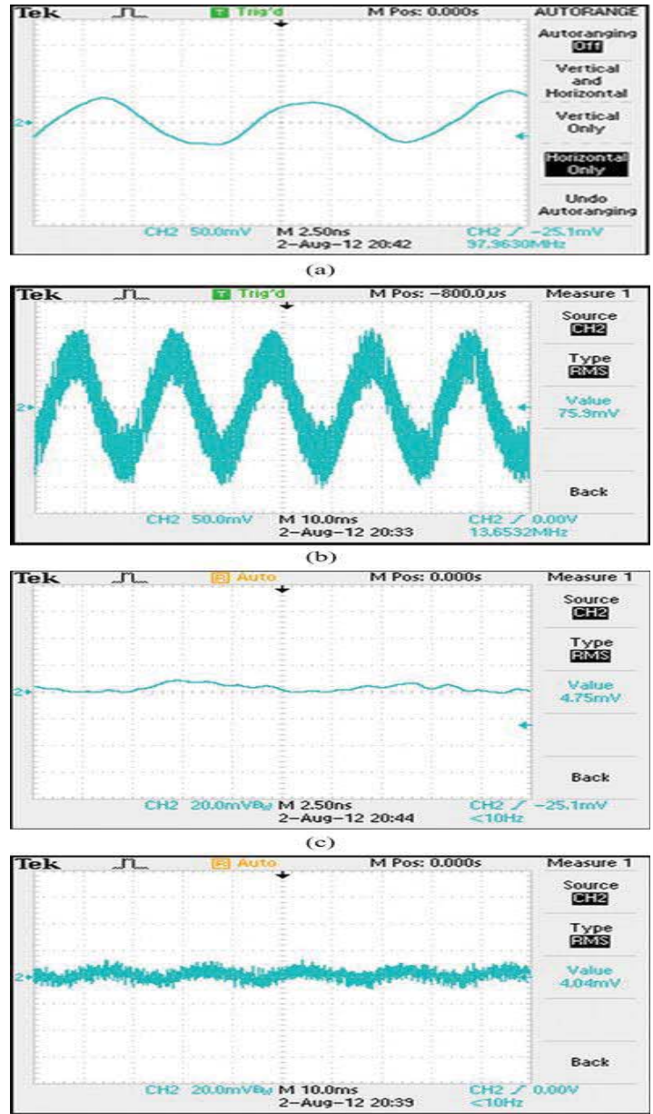
Fig. 7. (a) Output waveform of current transformer for different appliances. Output waveform of current transformer for 100 W electric bulb, (b) output waveform of current transformer for 800 W room heater, (c) output waveform of current transformer for 60 W electric bulb, and (d) output waveform of current transformer for audio device.
