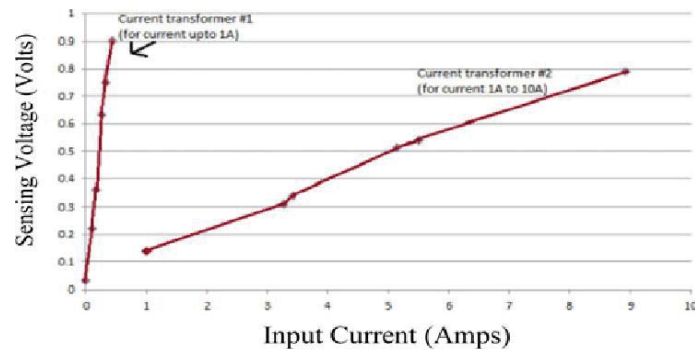
Fig. 5 scaling factor (m2) of current signal.
