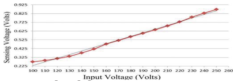
Fig. 4. Scaling factor ( m_1 ) of voltage signal. I_{act} = m_2 \times V_{measured\ voltage} for current
