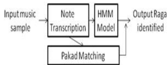
Fig. 3: HMM model and Pakad matching system.
