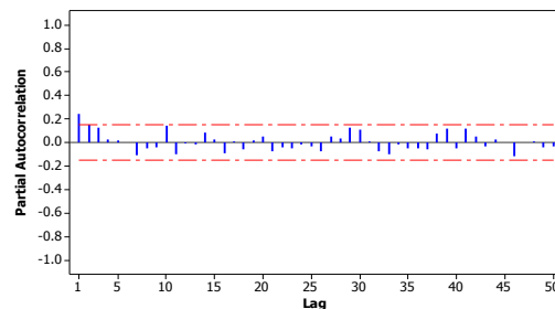
Figure 3. Scatter Plot Of PACF Of Wind Speed
