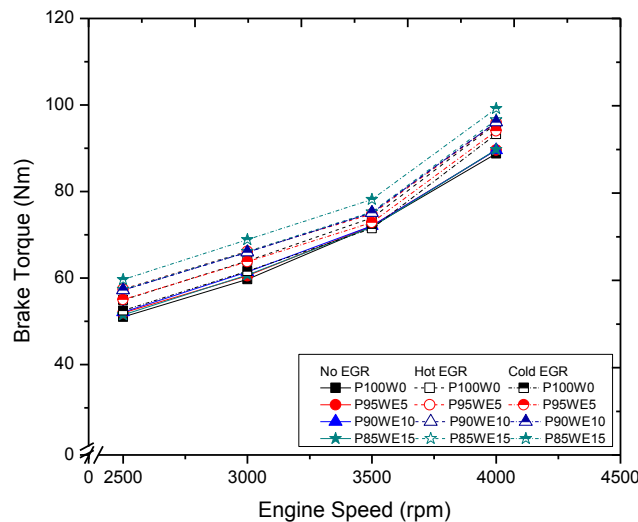
Figure 2. Brake torque for various fuel blends with or without EGR at variations in engine speed.
