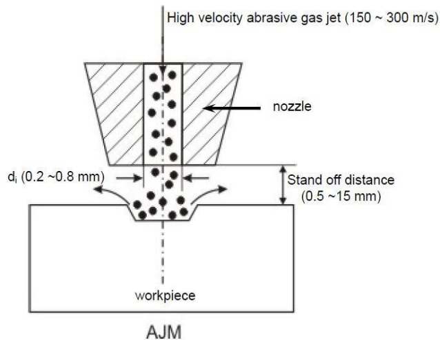
Fig.15 abrasive nozzle operation
