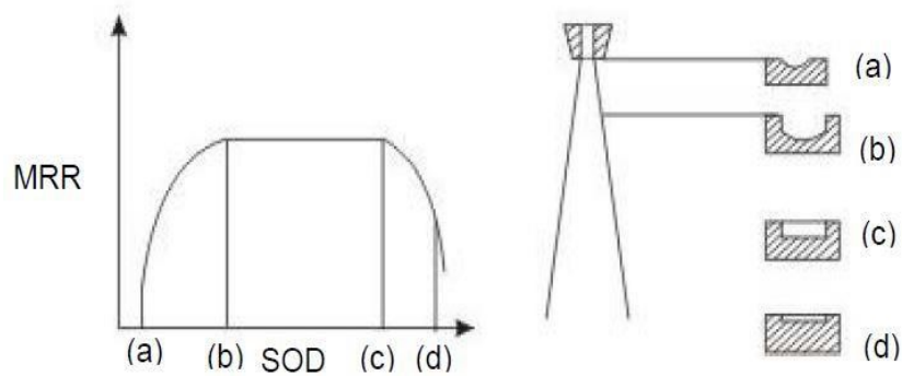
Fig.3 SODvs MRR
