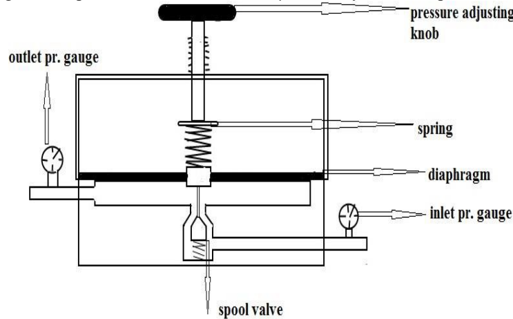
Fig.-14 Pressure regulator working
