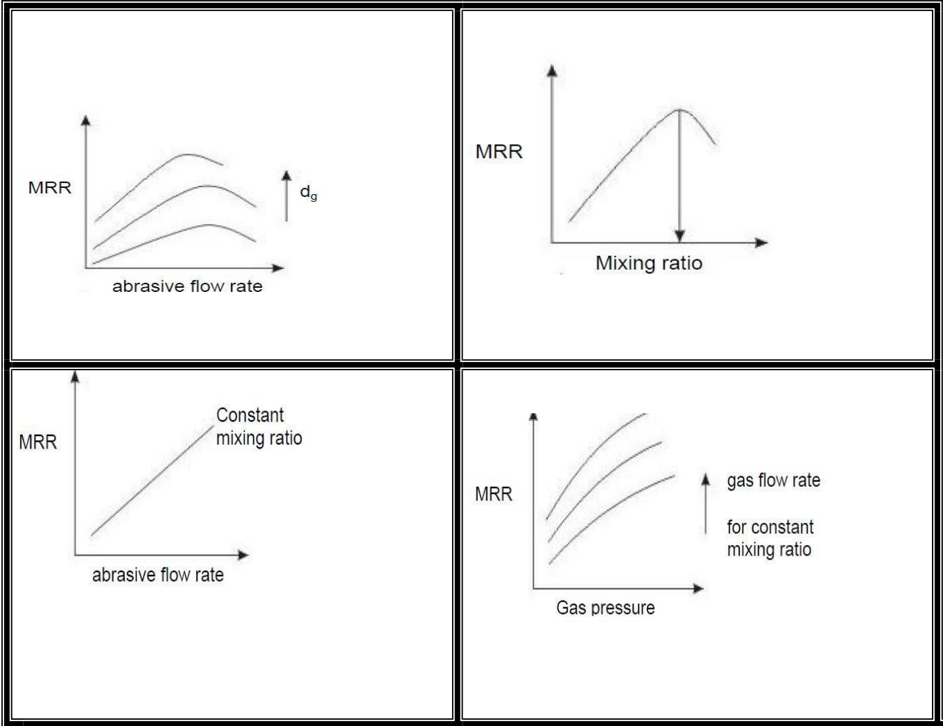
Fig.2-Operacting characteristics
