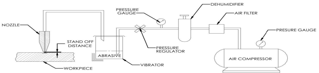
Fig-1- Layout of abrasive jet machine Performance
