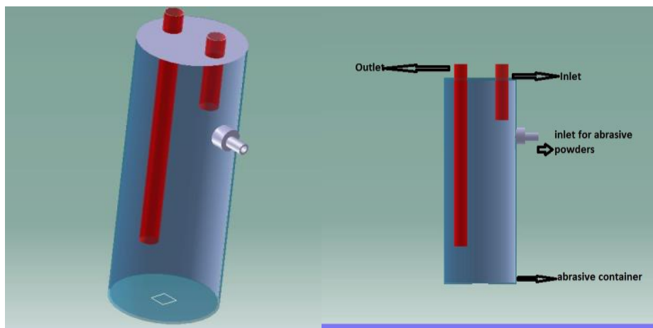
Fig.12 mixing chamber
