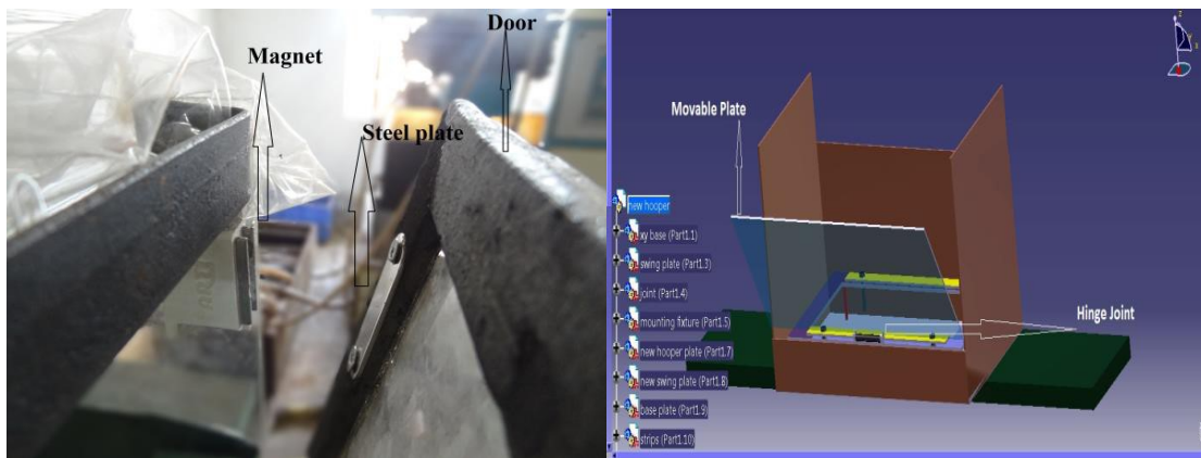
Fig-9 Magnetic clamp Fig-10 Door opening mechanism
