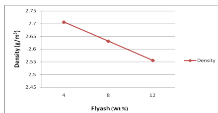
Figure 5. Density Vs Flyash
