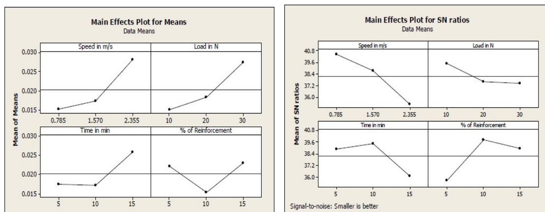
Figure. 6 Main Effects Plot for Means – Wear Rate & Coefficient of Friction for talc
